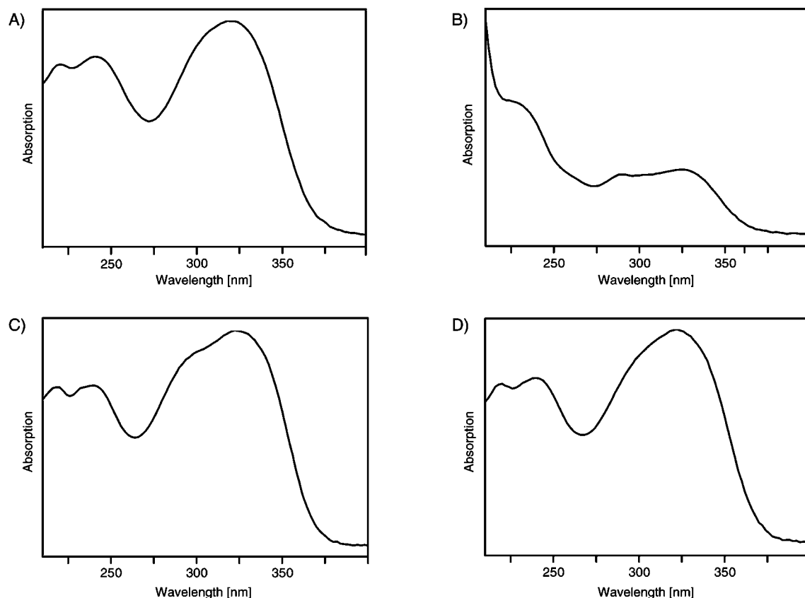
Figure 4. UV spectra of (A) compound 1 [8-5(noncyclic)/5-5-dehydrotriferulic acid], (B) compound 2 [8-8(tetrahydrofuran)/5-5-dehydrotriferulic acid], (C) compound 3 [4- O -8/5-8/ O -4-dehydrotetraferulic acid], and (D) compound 4 [4- O -8/5-5/8-5(noncyclic)-dehydrotetraferulic acid].
